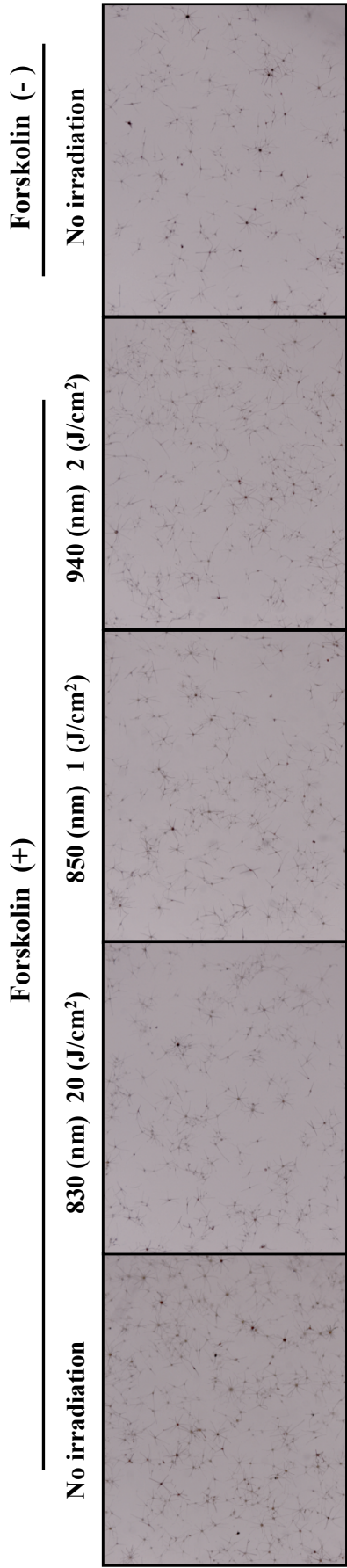
Fig. S2D. Effects of light-emitting diode wavelengths on cellular tyrosinase activity were determined according to L-DOPA stainability.
