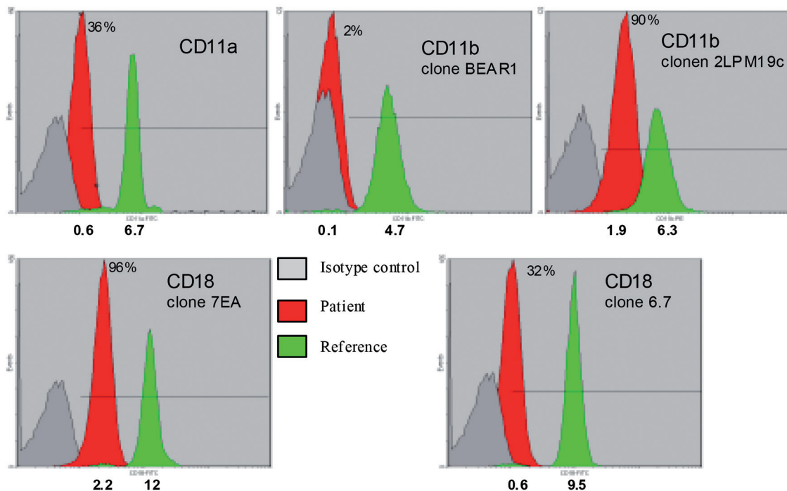
Fig. S2. Cell surface expression of \beta_2 -integrins on granulocytes from the patient and a healthy individual analysed by flow cytometry. The relative number (%) of granulocytes from the patient with an expression above background (isotype control) and the mean fluorescence intensity of the granulocyte population of the patient and reference are depicted. The horizontal line indicates expression above background. Analysis performed in January 2008. For details see Appendix S1 1 .
