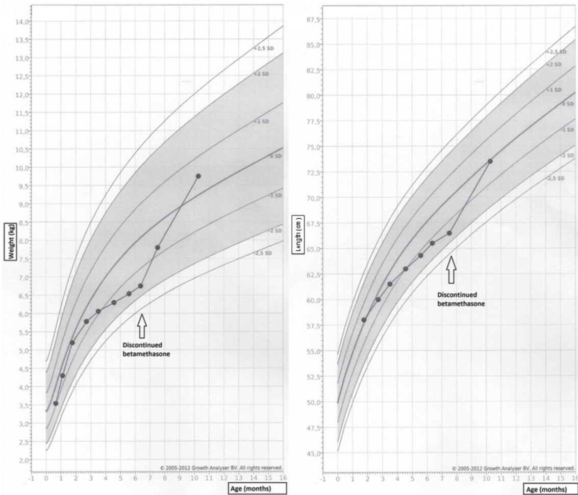
Fig. S1. Growth failure in Cushing's syndrome. Characteristic growth failure is evident on observing the patient's weight and length longitudinal growth curves.
