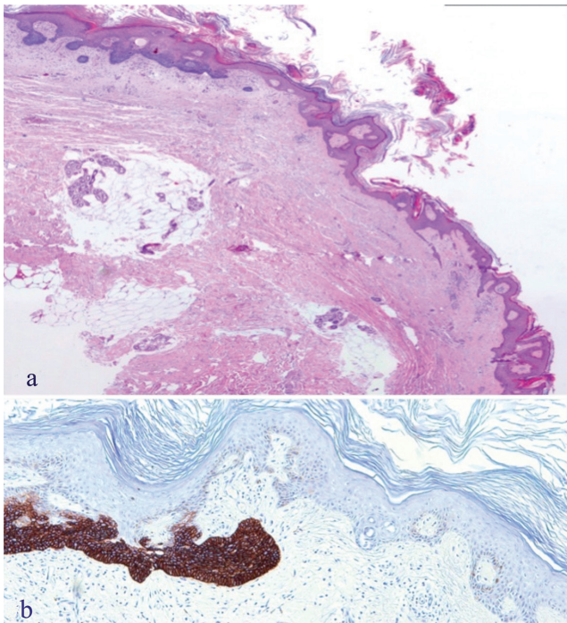
Fig. S1. a) Acanthosis, papillomatosis and hyperkeratosis typical of non-organoid non-epidermolytic epidermal naevi and nests of basaloid cells with a palisade pattern and hyperchromatic nuclei in the context of linear naevus (hematoxylin-eosin, magnification \times 4 ). b) Immunohistochemistry with BerEP4 showed areas of basaloid differentiation at the periphery of the lesion, without involvement of the epidermis not affected by BCC (magnification \times 10 ).
