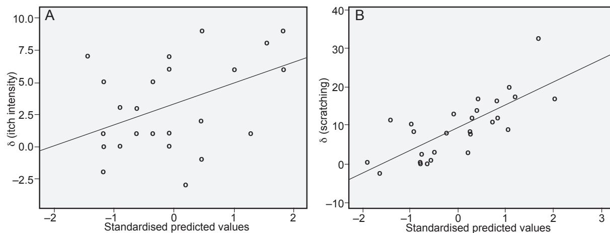
Fig. S1. Stepwise linear regression analyses. Depression was a significant predictor of self-rated induced itch in patients with atopic dermatitis (AD) ( n=27 ; corrected R^2=0.175 ) (A), while agreeableness and public self-consciousness were significant predictors of induced scratch movements in this patient group ( n=27 ; corrected R^2=0.534 ) (B).
