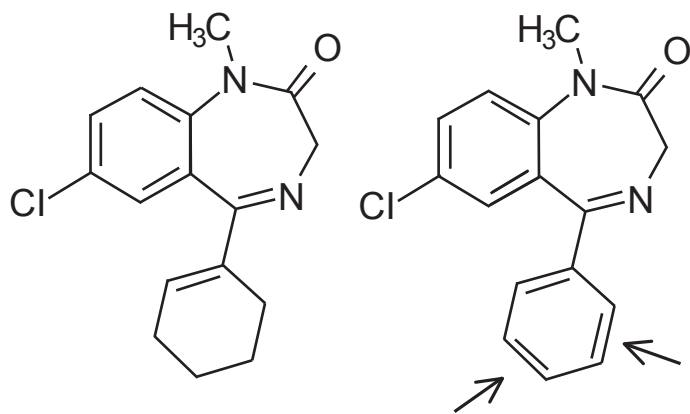
Fig. S1. Structural chemical formula of tetrazepam (left) and diazepam (right). Differences indicated by arrows (9).
