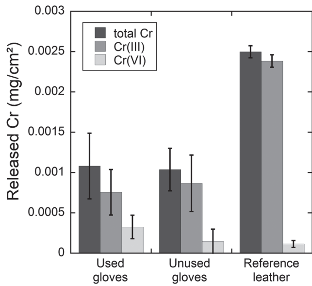
Fig. S1. Chromium Cr(III), Cr(VI), and total Cr released from used ( n=5 ) and unused ( n=5 ) gloves, and the Cr-tanned reference sample ( n=3 ), normalized to the surface area of the leather ( \text{mg}/\text{cm}^2 ).
