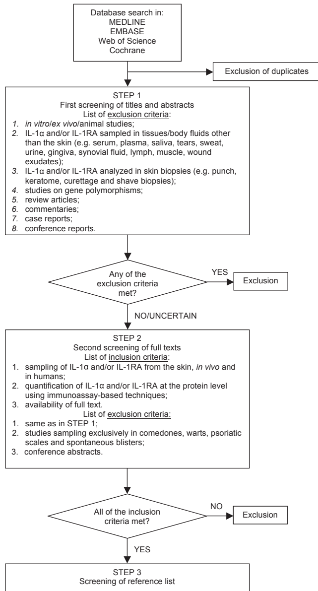
Fig. S1. Selection process. IL-1 \alpha : interleukin-1 \alpha ; IL-1RA: interleukin-1 receptor antagonist.
