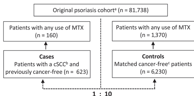
Fig. S1. Study flow chart. a Patients \geq 18 years \geq 2 outpatient psoriasis diagnoses in the period 2001 to 2016. At least one of the diagnoses needed to be made by a dermatologist. All patients had to live in Sweden from the start of the Swedish drug prescription registry (i.e. July 2005) to the index dates. The index date was in the period 2010 to 2016. b Patients with a first cSCC in the period 2010 to 2016. Prior to the cSCC diagnosis, the cases needed to be cancer-free, with the exception of basal cell carcinoma (BCC). c The controls needed to be alive and cancer-free (with the exception of BCC) on the index date. The matching criteria were age (same birth year) and sex. The controls were drawn from the group of eligible patients using risk set sampling. cSCC: cutaneous squamous cell carcinoma including squamous cell carcinoma in situ ; MTX: methotrexate.
