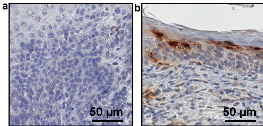
Fig. S1. Immunohistochemical staining for murine cathelicidin-related antimicrobial peptide (CRAMP) demonstrating lack of expression in the tail skin of (a) C57BL/6J mouse deficient for CRAMP, in contrast to a (b) C57BL/6J wild-type control mouse.
