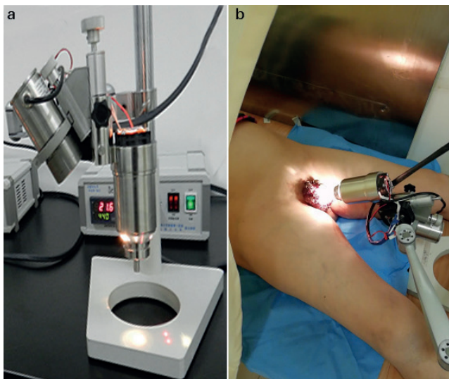
Fig. S2. Hyperthermia device and procedure. (a) Patented hyperthermia device with a light source from a tungsten-halogen lamp. With this device it was possible to ensure that the local hyperthermia delivered the required temperature (44°C) at the lesion site. (b) Local hyperthermia treatment procedure.
