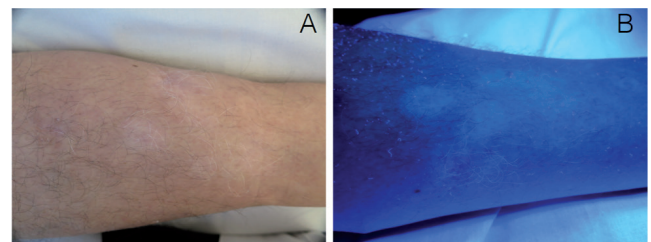
Fig. 1. Case 1. (A) Well-defined hypochromic lesions with non-pigmented hairs on the pretibial area. Those lesions appeared at the sites of the previous melanoma metastases. (B) At 20 months from the complete response the vitiligo plaques were still visible and stable in size, as seen under Wood's lamp.
