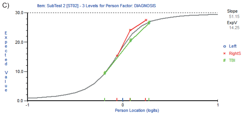
Figure S2C. DIF plot for Communication super-item for TBI and right stroke samples.
