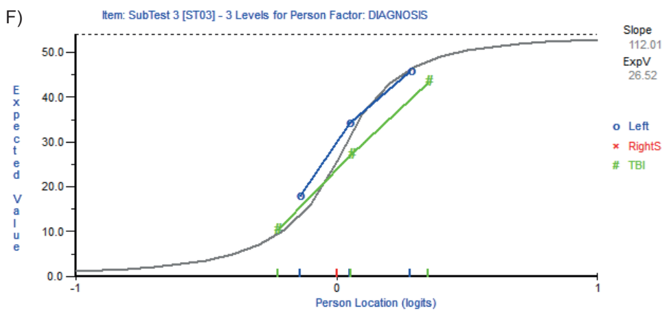
Figure S2F. DIF plot for Psychosocial super-item for TBI and left stroke samples.
