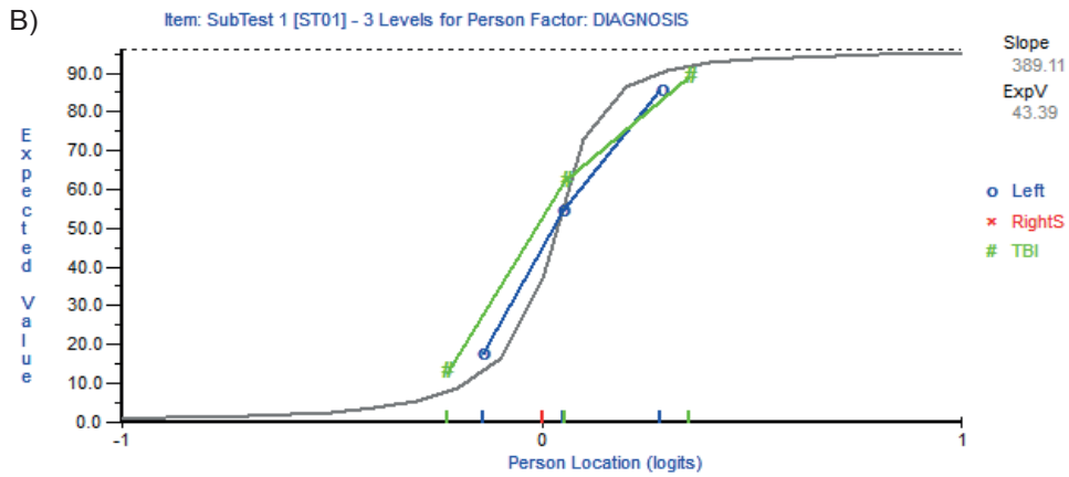
Figure S2B. DIF plot for Motor super-item for TBI and left stroke samples.
