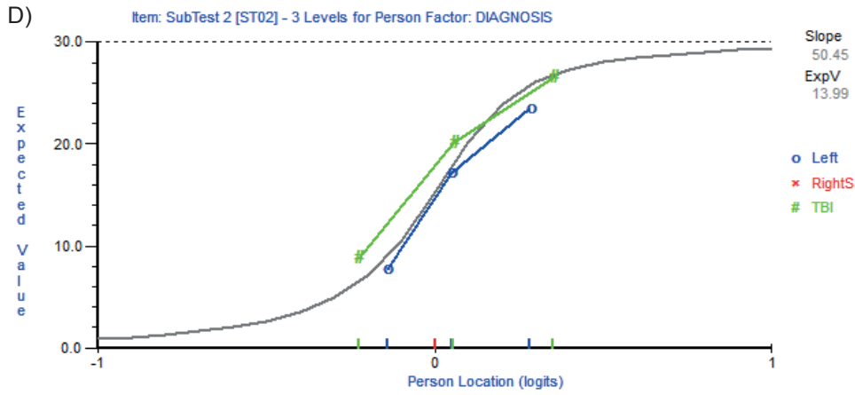
Figure S2D. DIF plot for Communication super-item for TBI and left stroke samples.
