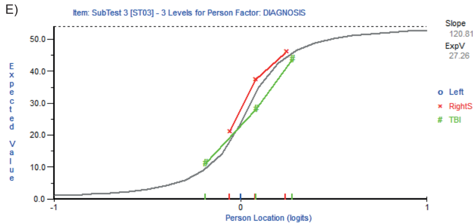
Figure S2E. DIF plot for Psychosocial super-item for TBI and right stroke samples.
