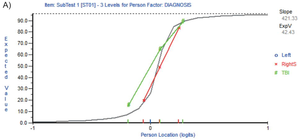
Figure S2A. DIF plot for Motor super-item for TBI and right stroke samples.
