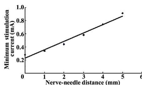
Fig. 1. Relationship between nerve–needle distance and required current. Linear regression analysis shows a linear relationship between nerve–needle distance ( X ) and minimum current ( Y ). The linear equation is Y = 0.13X + 0.22 ( r^2 = 0.974 , p < 0.05 ).
