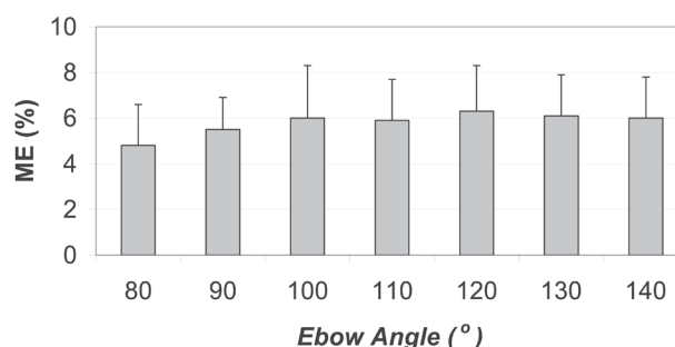
Fig. 2. Gross mechanical efficiency (ME) for 12 subjects with a spinal cord injury (mean (standard deviation) in association with seat height (expressed as elbow angle; full extension = 180°).
