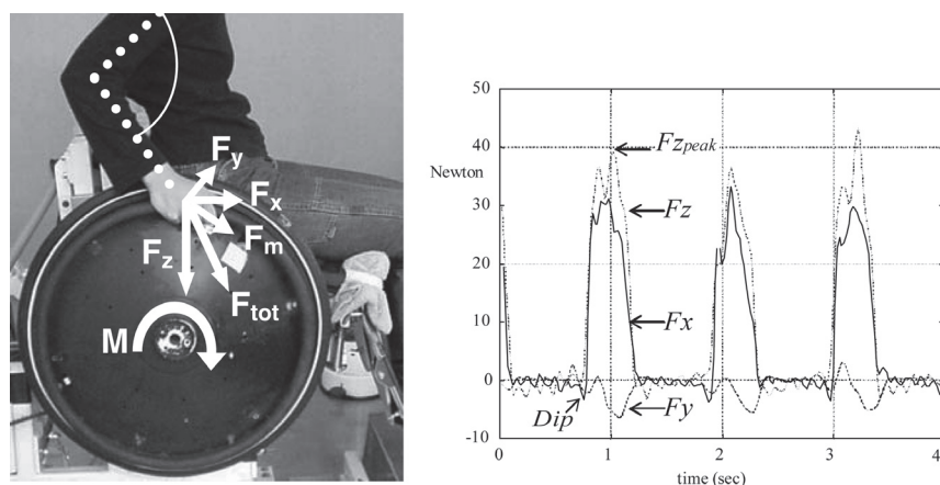
Fig. 1. Side view (left panel) of the computerized wheelchair ergometer set-up with graphics of force components and moments that can be derived from the ergometer measurement system (24, 38), as well as the upper and lower arm definition and elbow angle (.....), which was used for seat height adjustment (full extension = 180°). In the right panel typical time tracings of the separate F_x , F_y , F_z force components for 3 subsequent pushes are shown. F_m : tangential force onto the hand rim; M : torque around the wheel axle; F_{tot} : total force applied onto the hand rim; F_x , F_y , F_z : orthogonal force components of F_{tot} .
